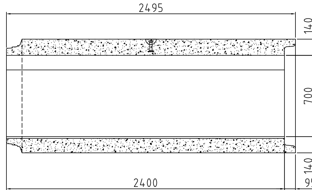
Joint section
