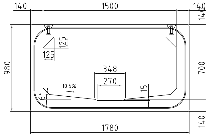
Socket view
