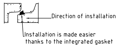
Joint section
